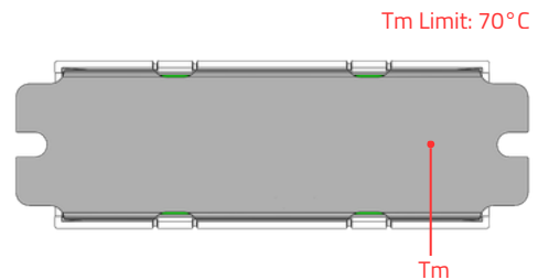
T_m is measured using a thermocouple placed on the center of the output-side bottom metal encasement while the device is mounted. Position the thermocouple between the bottom of the APT and the mounting surface, on the output connector side of the device.
