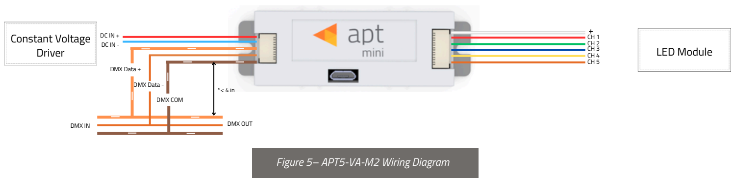
Figure 4 – APT3-VA-M2 Wiring Diagram
