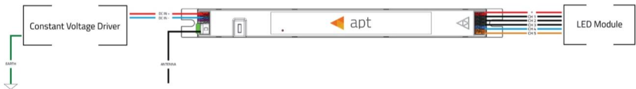
Figure 3 - APT-CV5-VWC Wireless Communication Configuration
