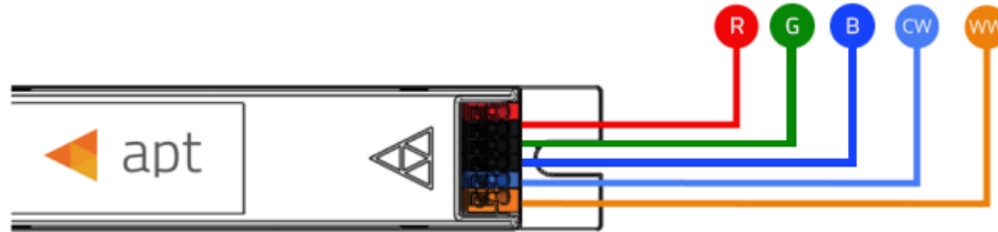
Figure 2 - Wiring APT-CV5-VA-LN to RGBWW LED Module
