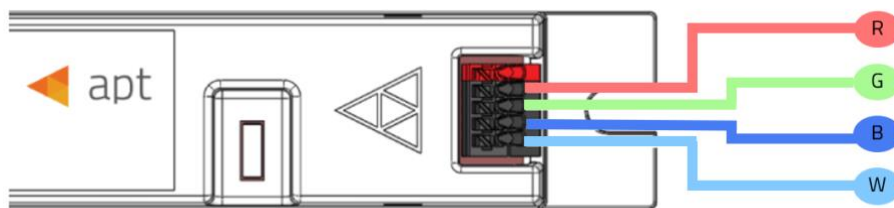
Figure 5 - Wiring APT-CV4-VWC-LN-CVO to RGBW LED module
