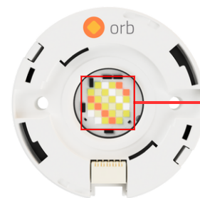
Figure 2 – To measure LED array surface temperature, use thermal camera with diffuser removed after system reached thermal equilibrium
